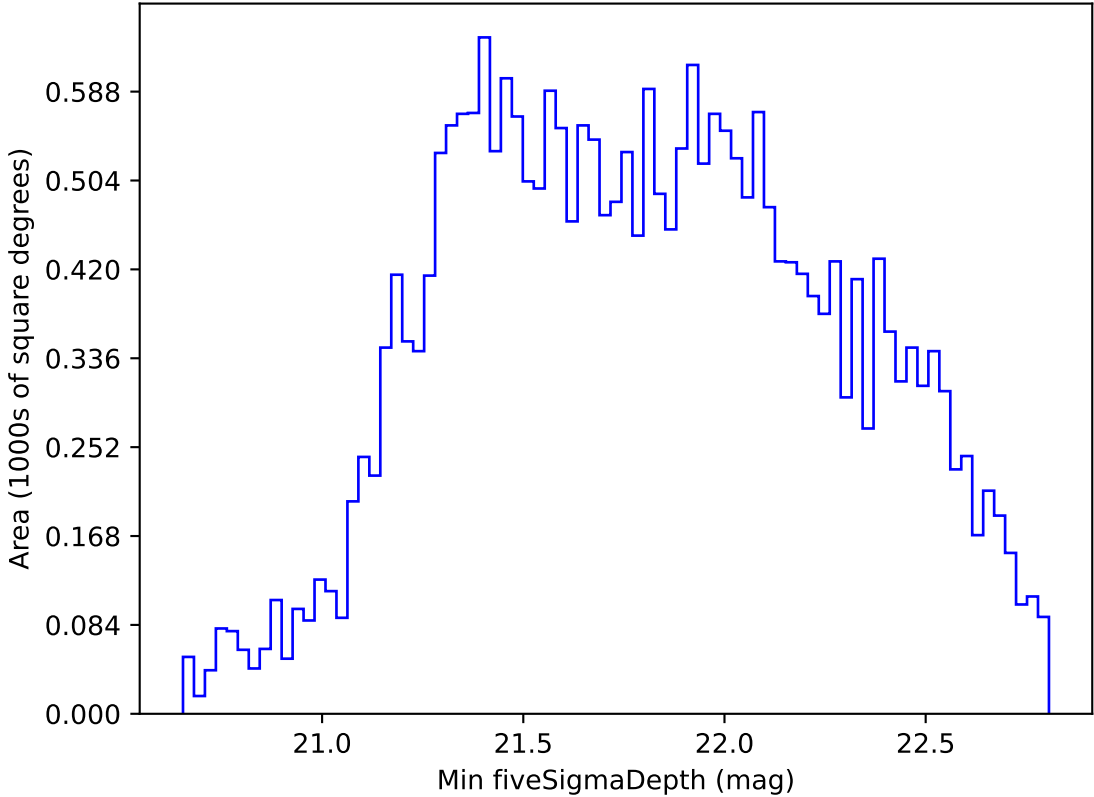
weather_cloudso4v3.4_10yrs All sky i band: Min fiveSigmaDepth
