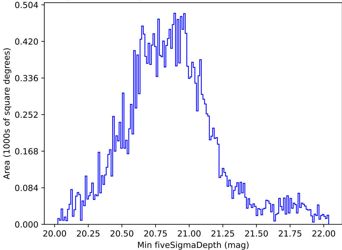
weather_cloudso4v3.4_10yrs All sky all bands: Min fiveSigmaDepth
