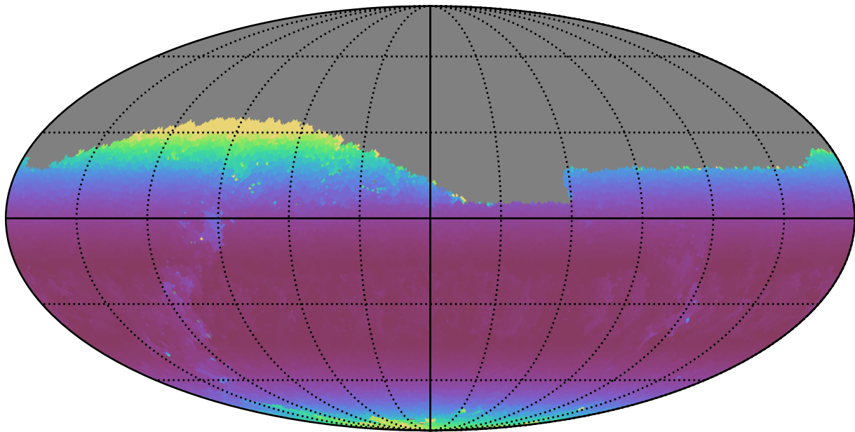
weather_cloudso4v3.4_10yrs Yr 1 z band: Min airmass
