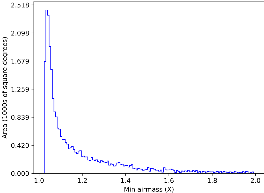
weather_cloudso4v3.4_10yrs Yr 1 z band: Min airmass
