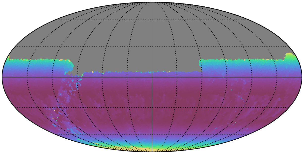
weather_cloudso4v3.4_10yrs Yr 1 y band: Min airmass
