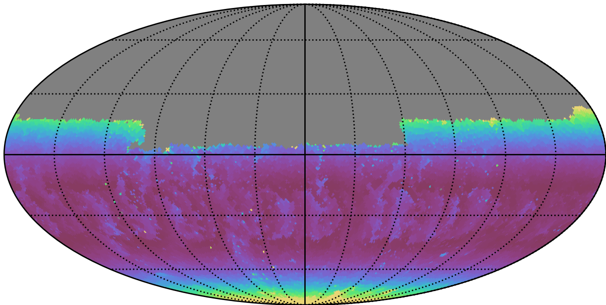
weather_cloudso4v3.4_10yrs Yr 1 u band: Min airmass
