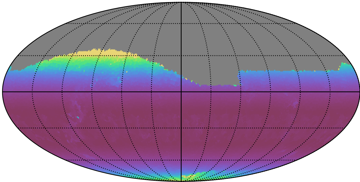
weather_cloudso4v3.4_10yrs Yr 1 r band: Min airmass
