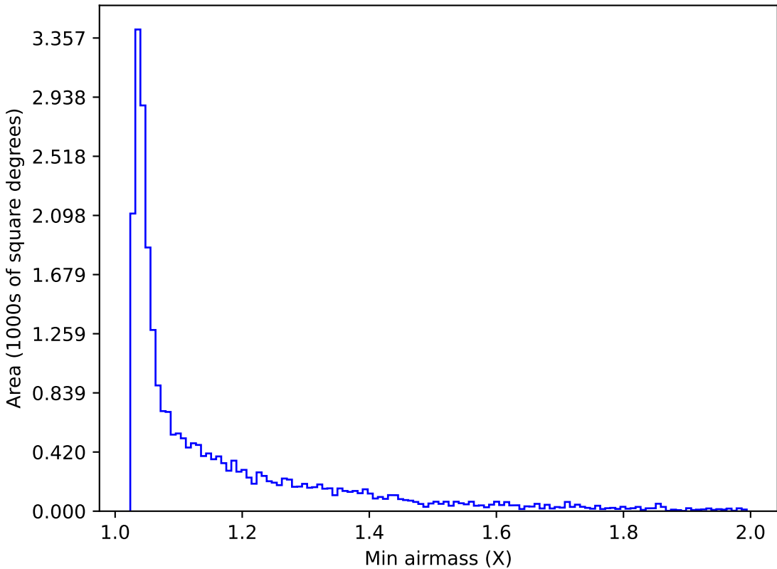
weather_cloudso4v3.4_10yrs Yr 1 r band: Min airmass
