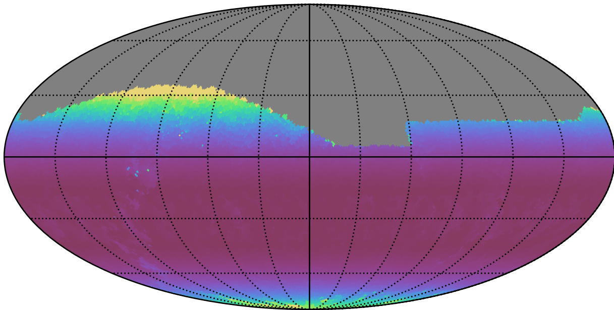
weather_cloudso4v3.4_10yrs Yr 1 i band: Min airmass
