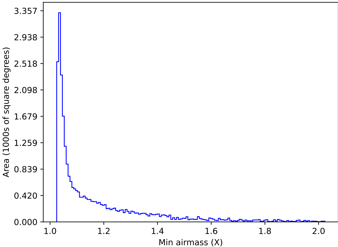
weather_cloudso4v3.4_10yrs Yr 1 i band: Min airmass
