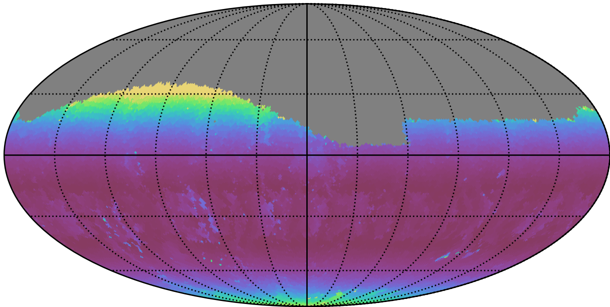
weather_cloudso4v3.4_10yrs Yr 1 g band: Min airmass
