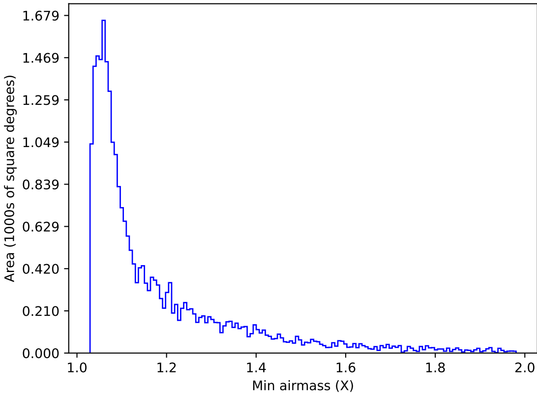
weather_cloudso4v3.4_10yrs Yr 1 g band: Min airmass
