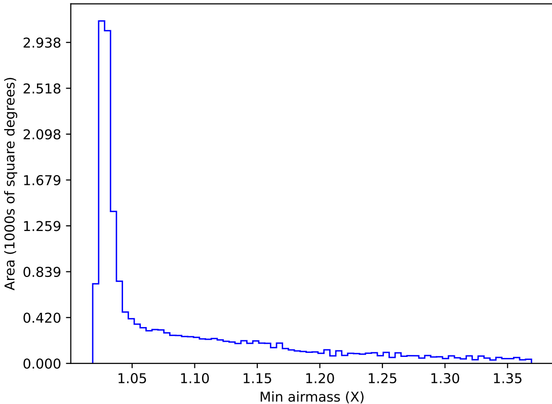
weather_cloudso4v3.4_10yrs WFD z band: Min airmass
