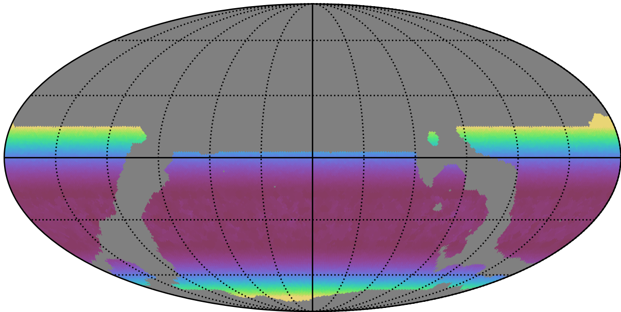
weather_cloudso4v3.4_10yrs WFD y band: Min airmass
