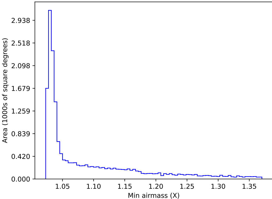
weather_cloudso4v3.4_10yrs WFD y band: Min airmass
