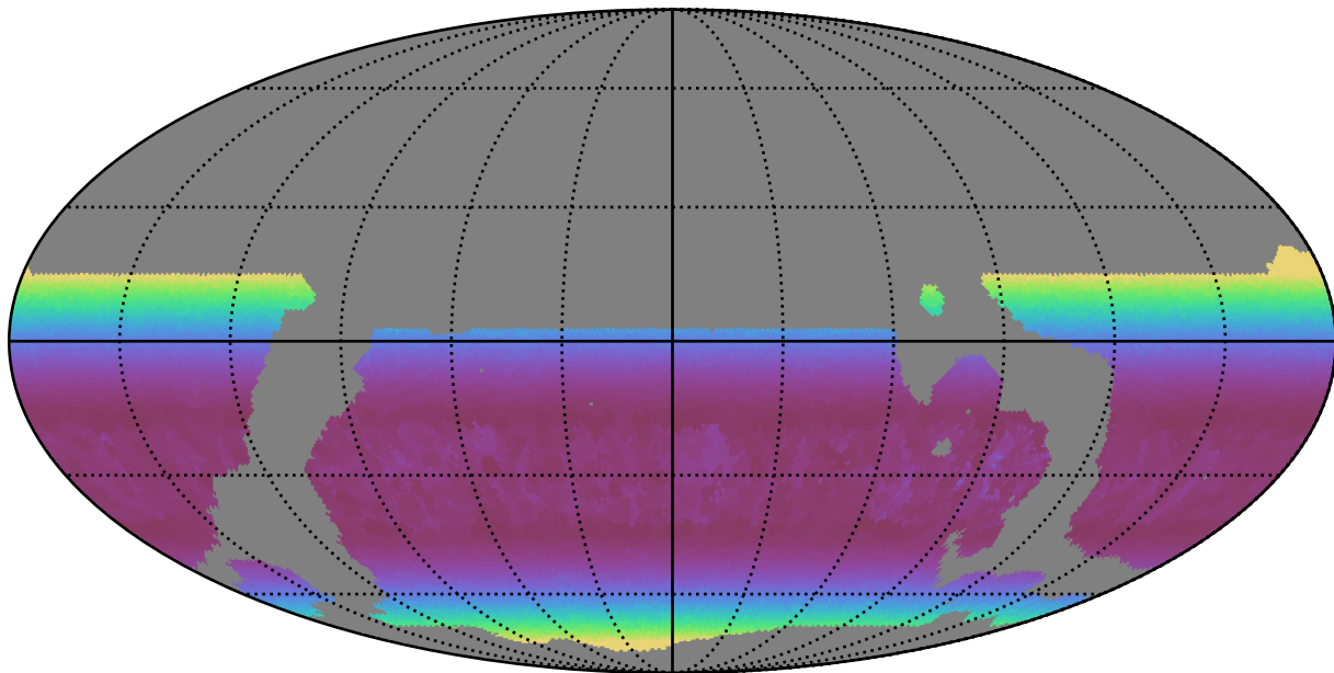
weather_cloudso4v3.4_10yrs WFD u band: Min airmass
