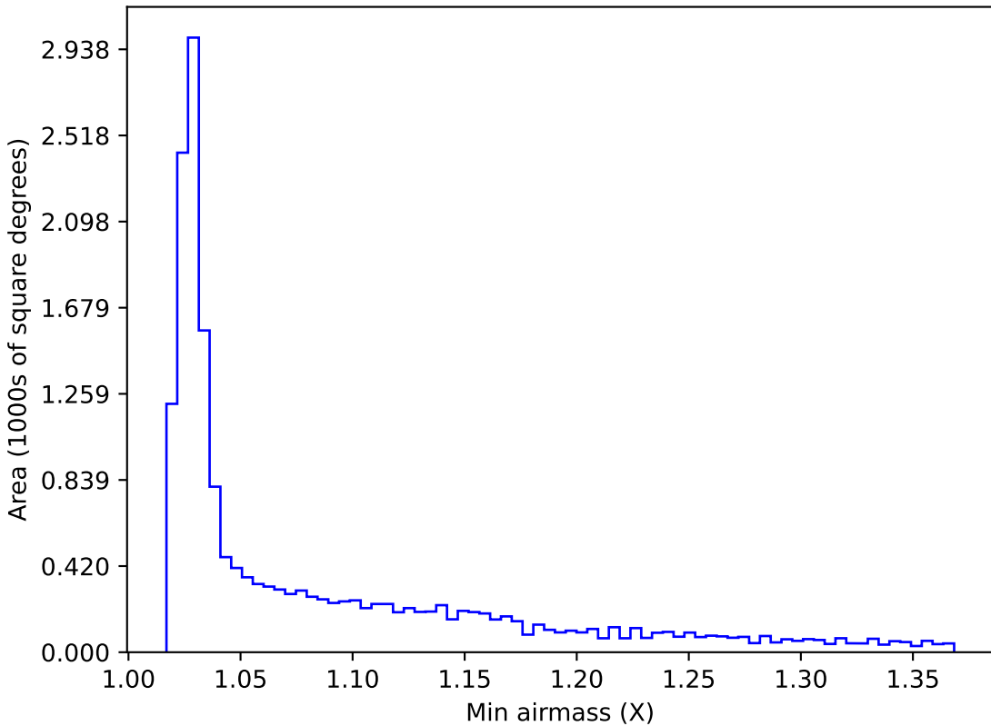
weather_cloudso4v3.4_10yrs WFD r band: Min airmass
