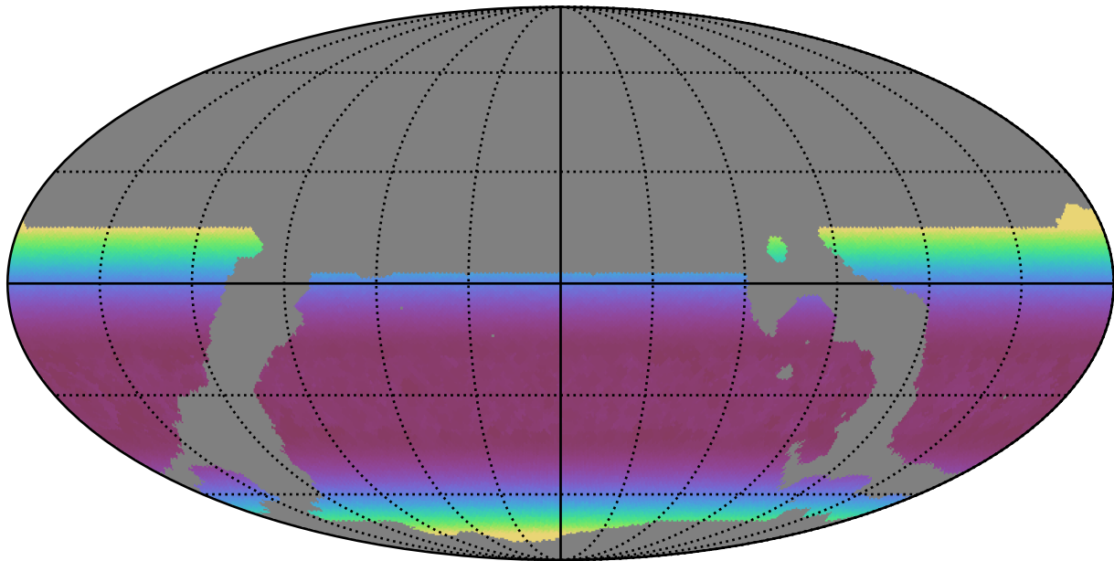
weather_cloudso4v3.4_10yrs WFD i band: Min airmass
