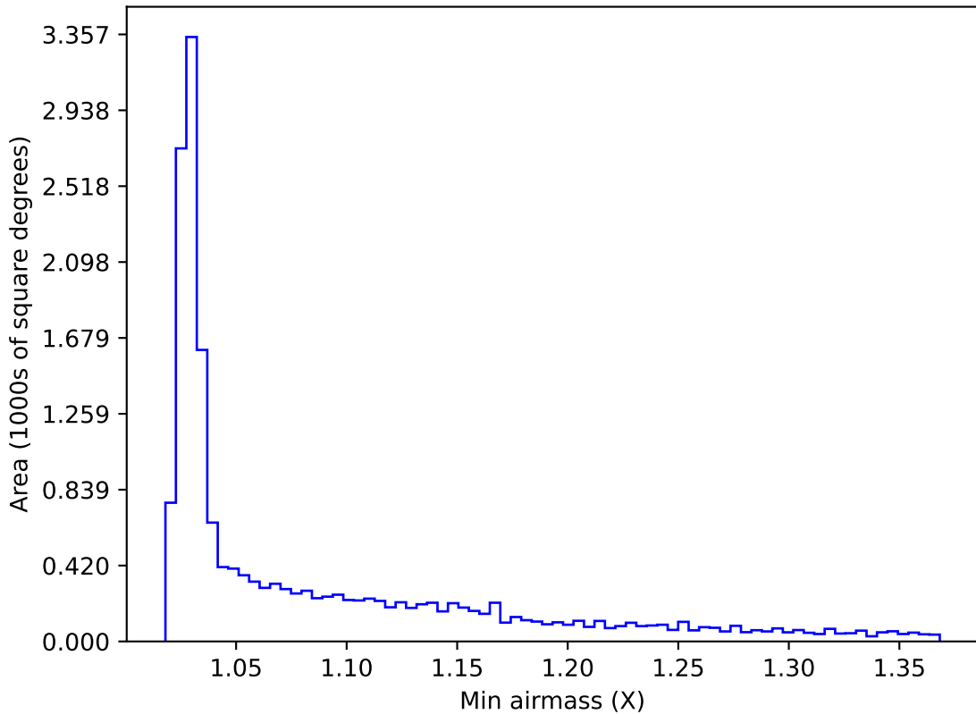
weather_cloudso4v3.4_10yrs WFD i band: Min airmass
