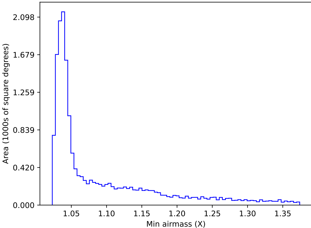
weather_cloudso4v3.4_10yrs WFD g band: Min airmass
