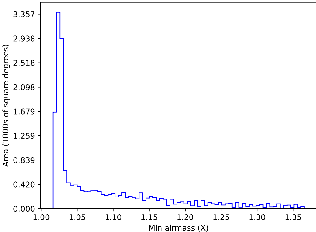
weather_cloudso4v3.4_10yrs WFD all bands: Min airmass
