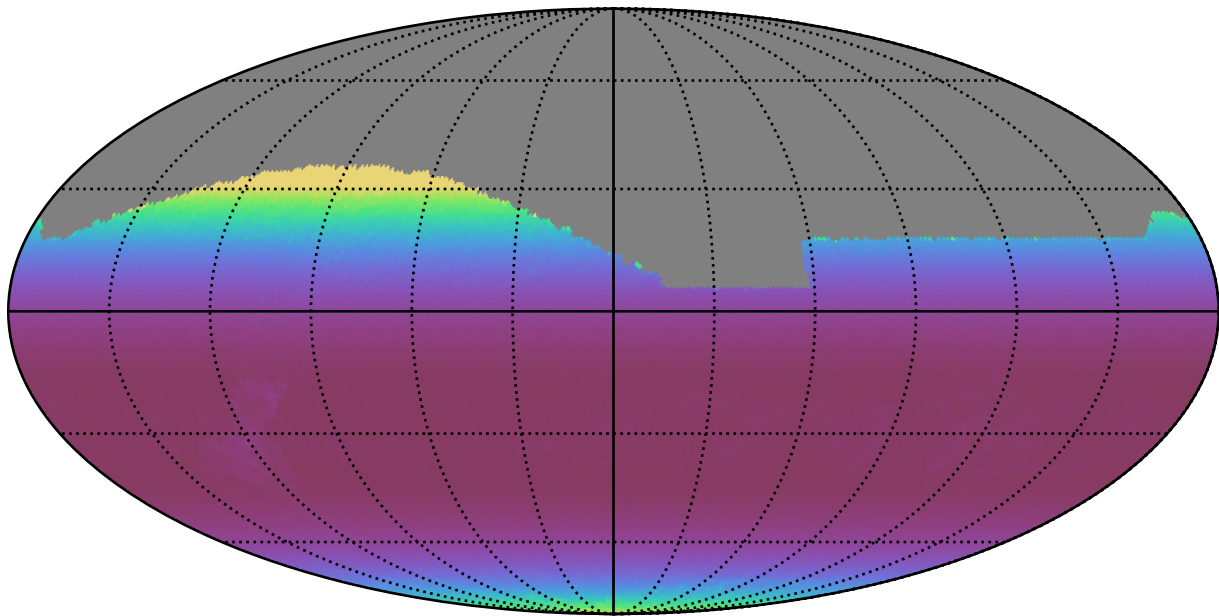
weather_cloudso4v3.4_10yrs All sky z band: Min airmass
