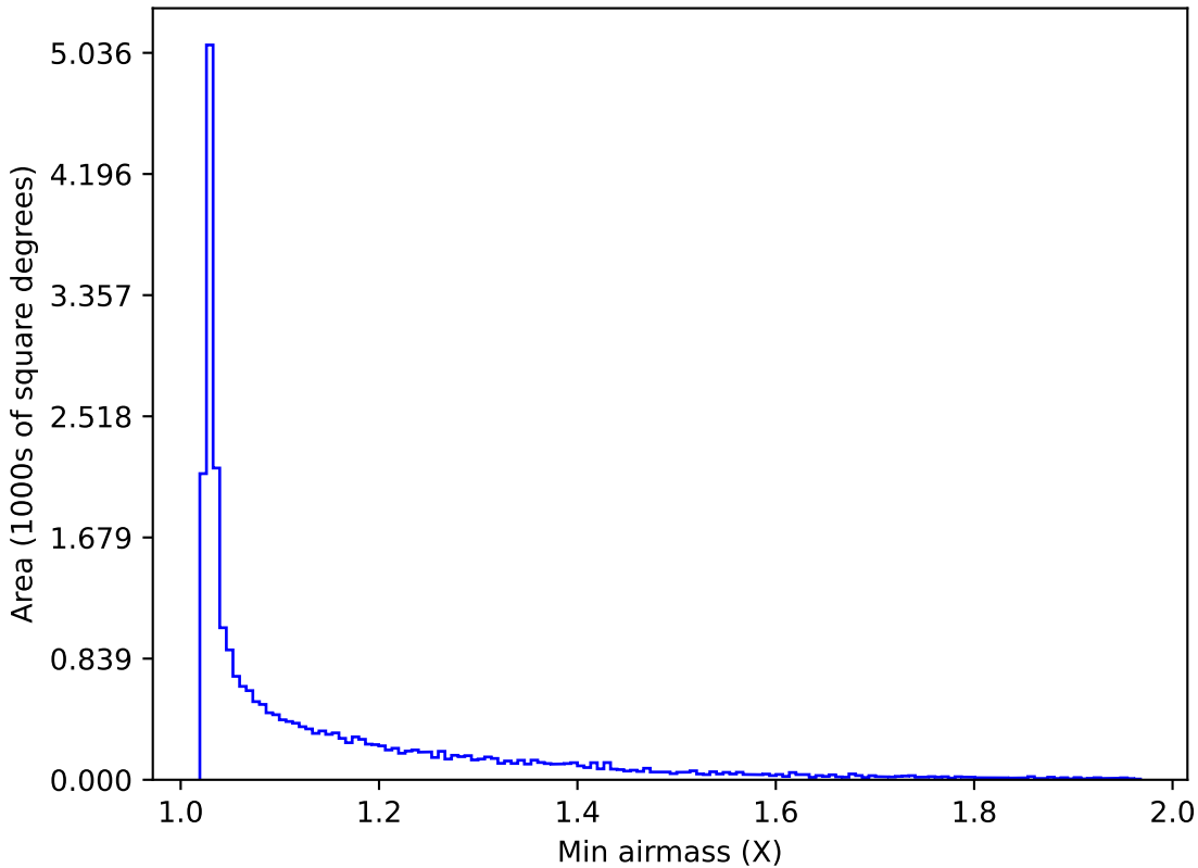
weather_cloudso4v3.4_10yrs All sky z band: Min airmass
