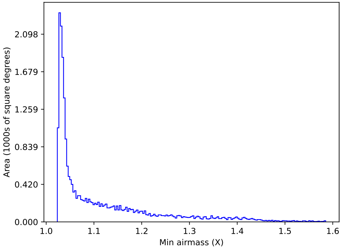
weather_cloudso4v3.4_10yrs All sky y band: Min airmass
