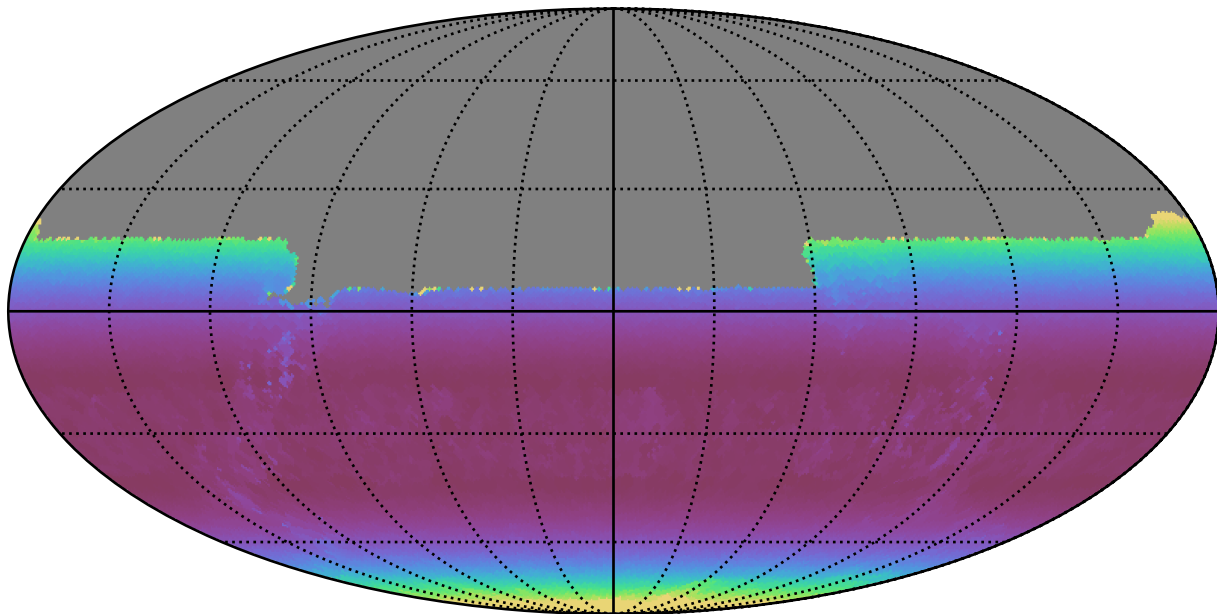
weather_cloudso4v3.4_10yrs All sky u band: Min airmass
