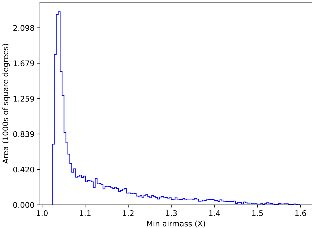
weather_cloudso4v3.4_10yrs All sky u band: Min airmass
