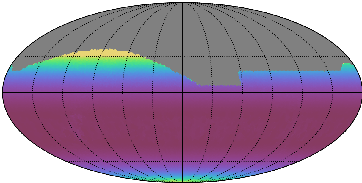
weather_cloudso4v3.4_10yrs All sky r band: Min airmass
