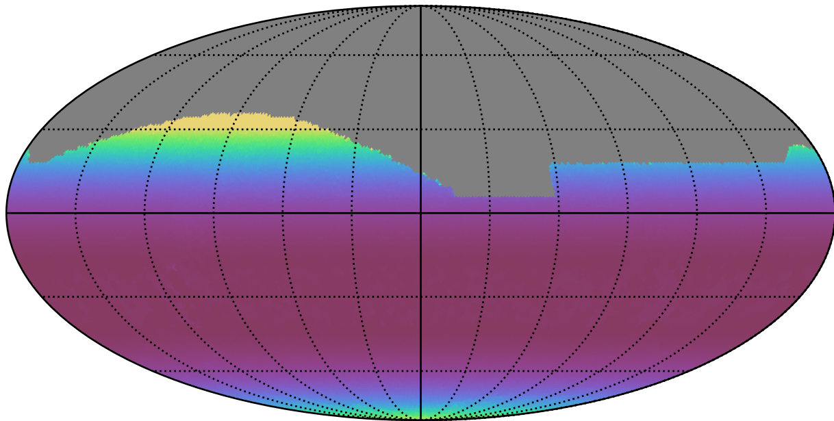
weather_cloudso4v3.4_10yrs All sky i band: Min airmass
