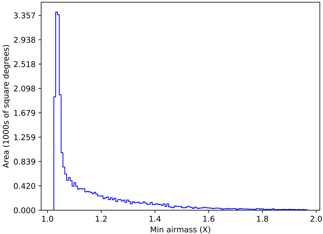
weather_cloudso4v3.4_10yrs All sky g band: Min airmass
