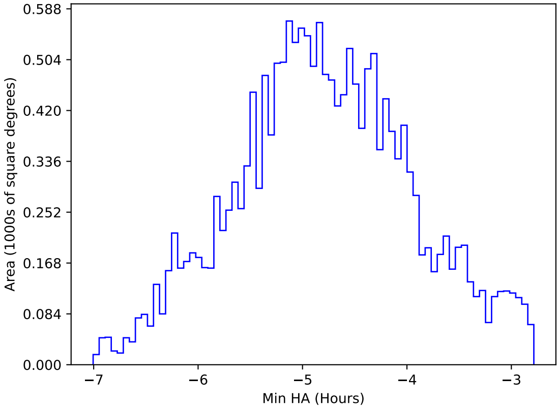
weather_cloudso4v3.4_10yrs WFD all bands: Min HA
