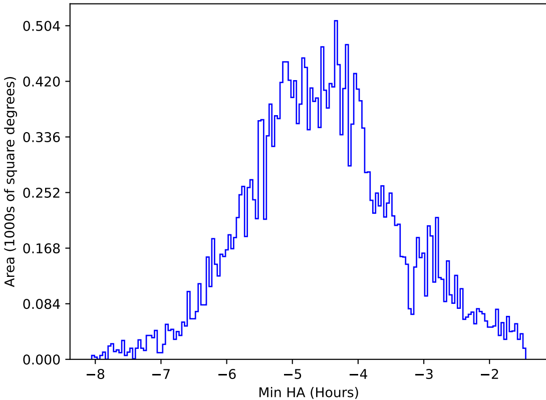
weather_cloudso4v3.4_10yrs All sky all bands: Min HA
