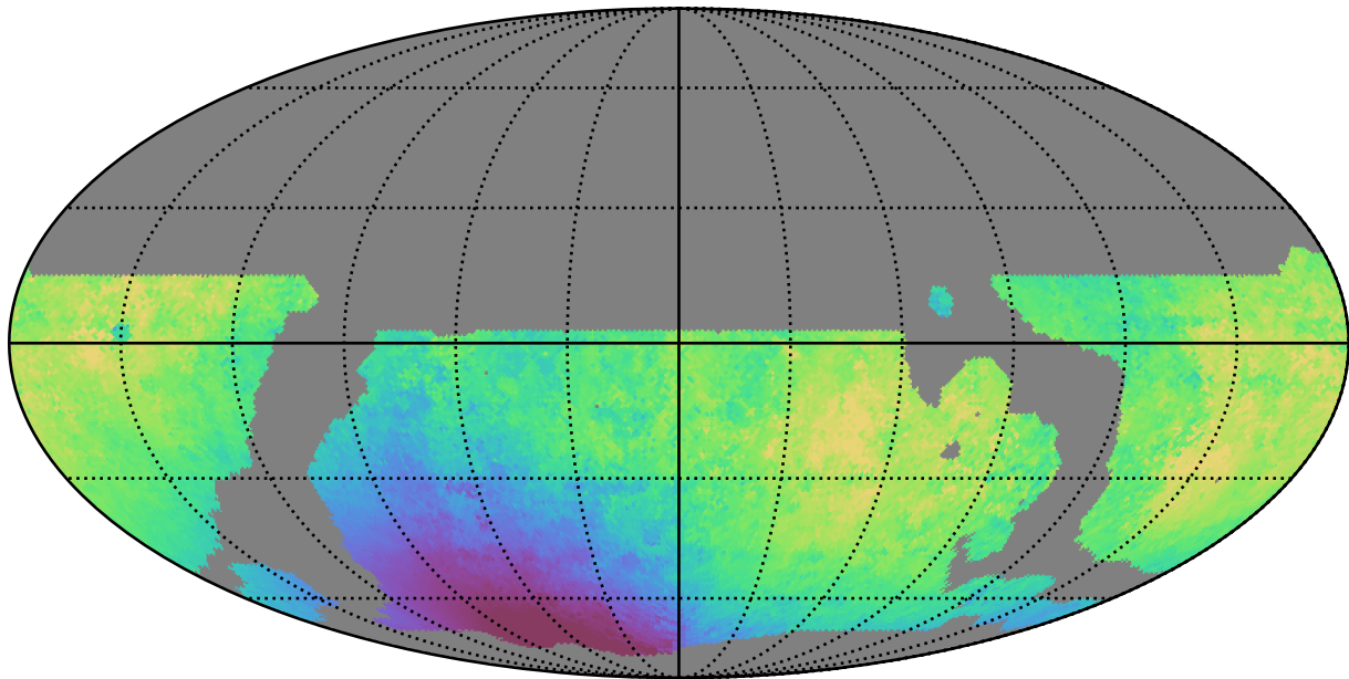
weather_cloudso4v3.4_10yrs WFD y band: Median solarElong
