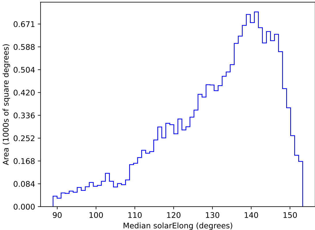
weather_cloudso4v3.4_10yrs WFD u band: Median solarElong
