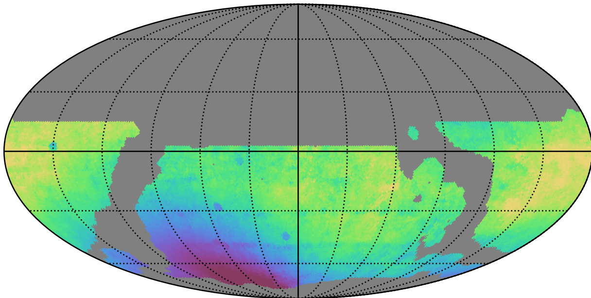
weather_cloudso4v3.4_10yrs WFD r band: Median solarElong
