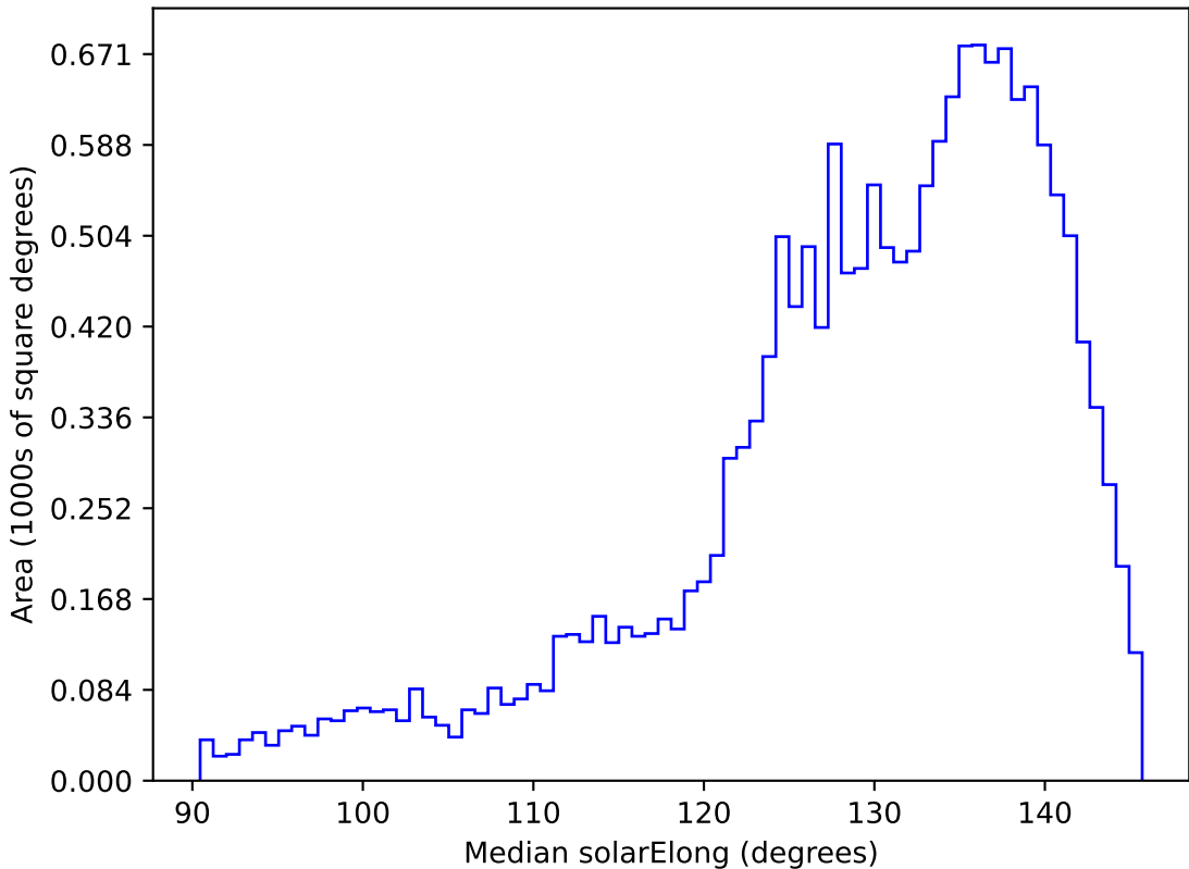
weather_cloudso4v3.4_10yrs WFD i band: Median solarElong
