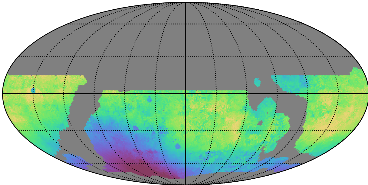
weather_cloudso4v3.4_10yrs WFD g band: Median solarElong
