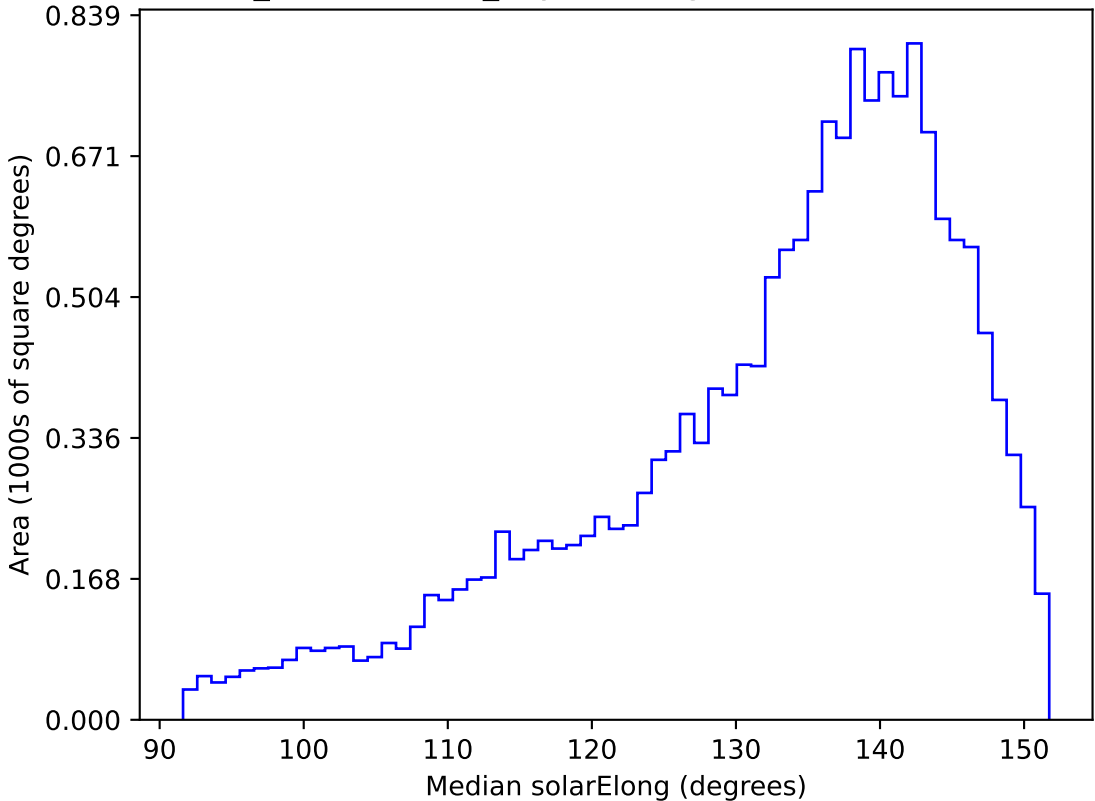
weather_cloudso4v3.4_10yrs WFD g band: Median solarElong
