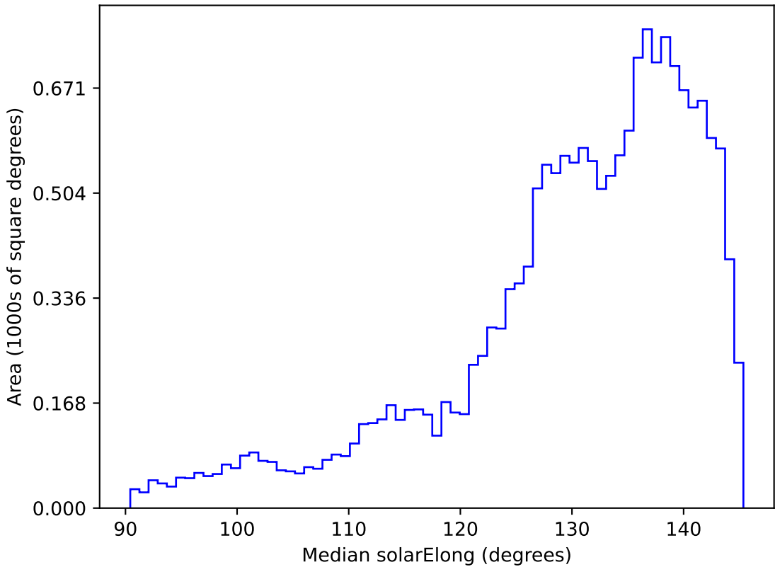
weather_cloudso4v3.4_10yrs WFD all bands: Median solarElong
