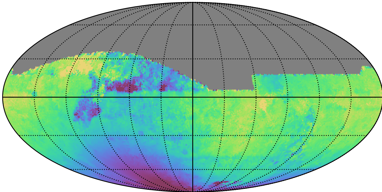
weather_cloudso4v3.4_10yrs All sky z band: Median solarElong
