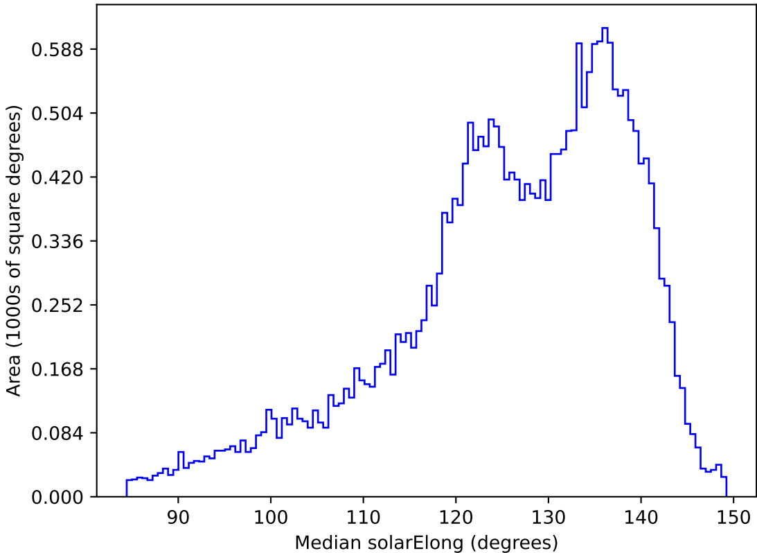
weather_cloudso4v3.4_10yrs All sky z band: Median solarElong
