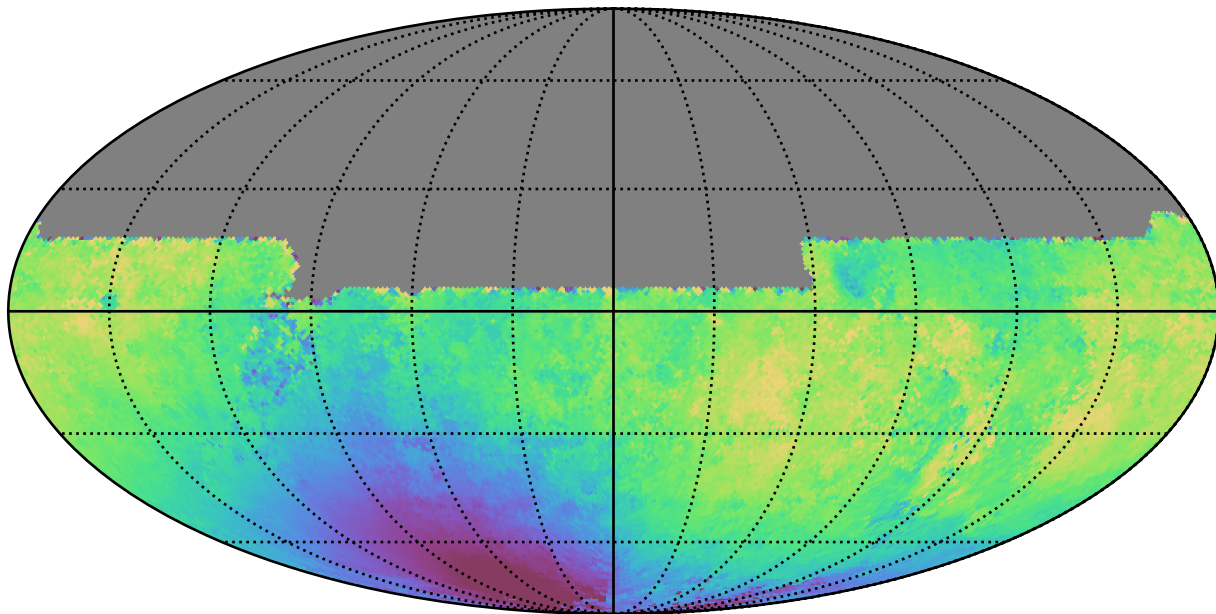
weather_cloudso4v3.4_10yrs All sky y band: Median solarElong
