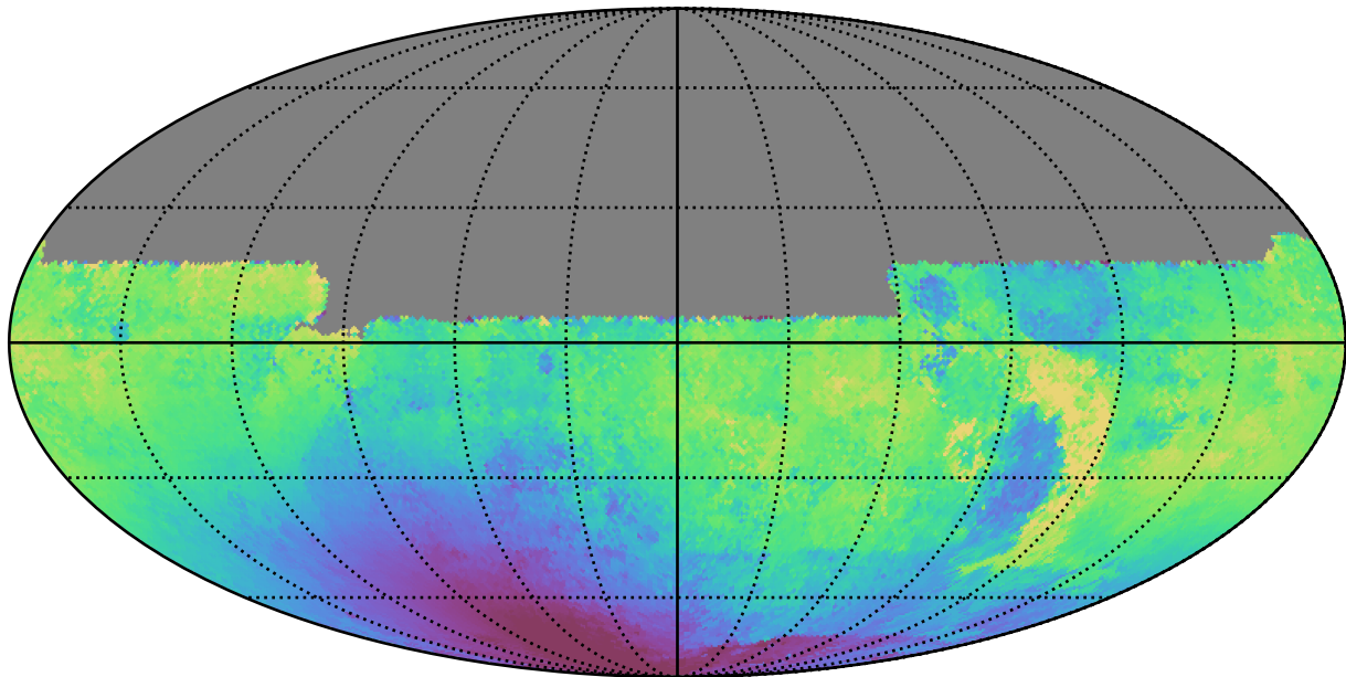
weather_cloudso4v3.4_10yrs All sky u band: Median solarElong
