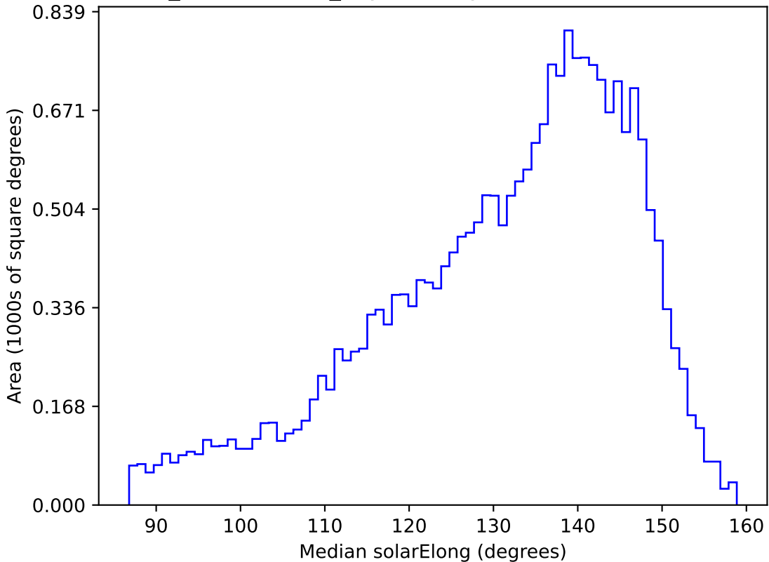
weather_cloudso4v3.4_10yrs All sky u band: Median solarElong
