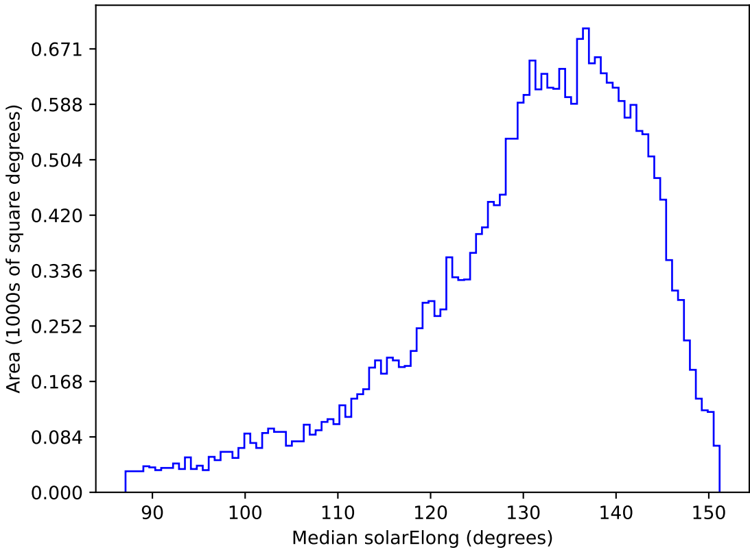
weather_cloudso4v3.4_10yrs All sky r band: Median solarElong
