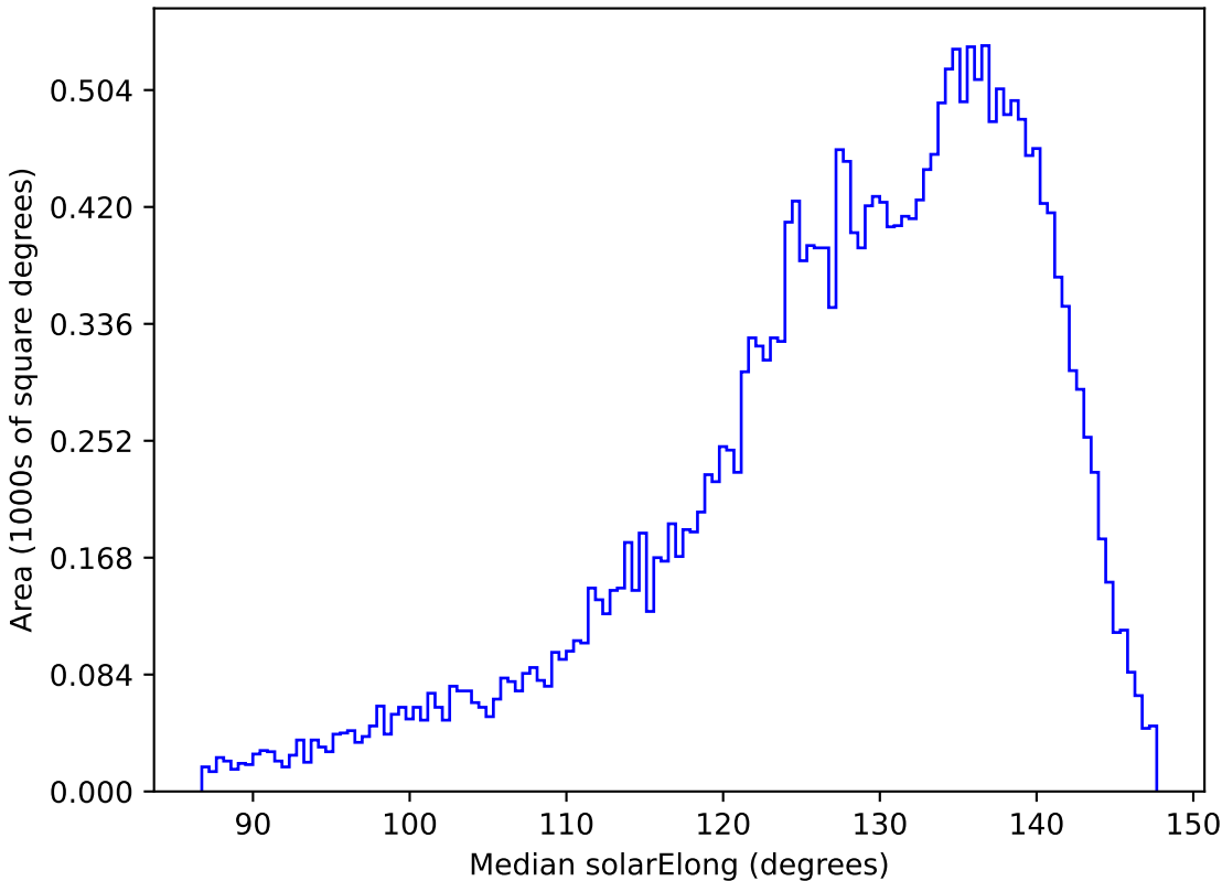
weather_cloudso4v3.4_10yrs All sky i band: Median solarElong
