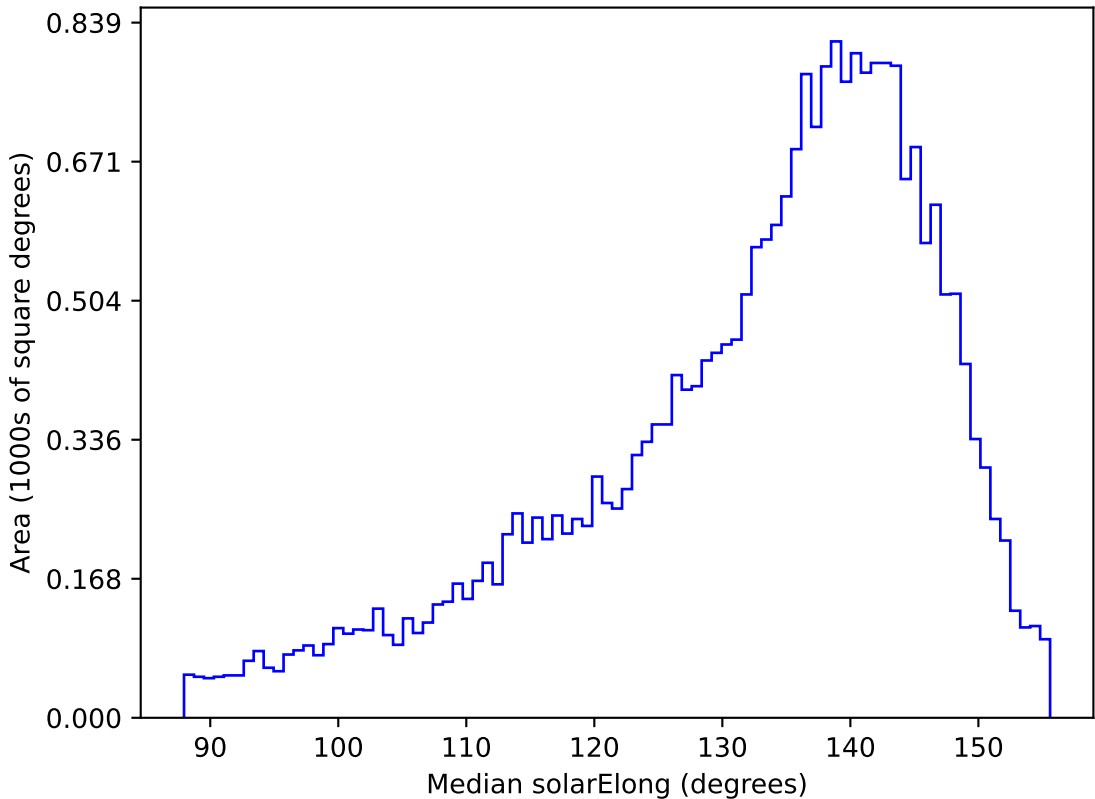
weather_cloudso4v3.4_10yrs All sky g band: Median solarElong
