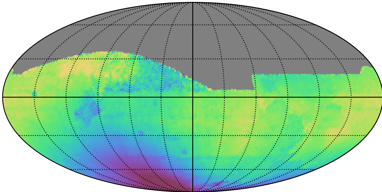
weather_cloudso4v3.4_10yrs All sky all bands: Median solarElong
