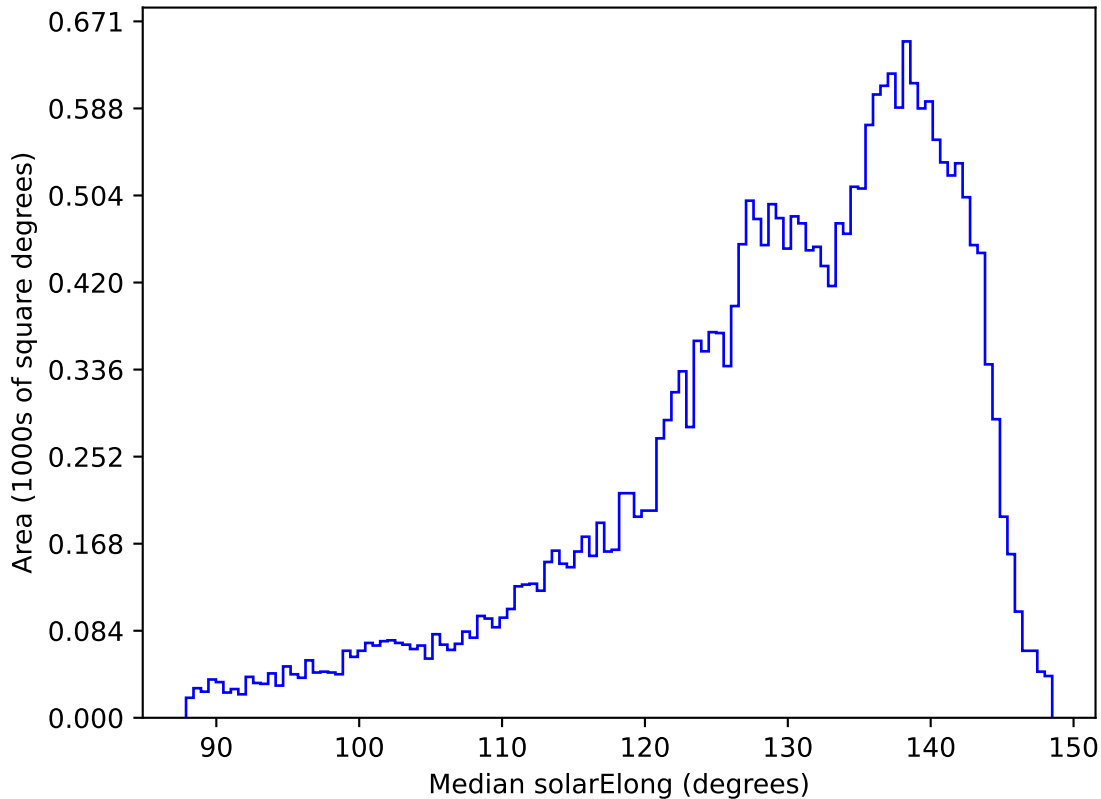
weather_cloudso4v3.4_10yrs All sky all bands: Median solarElong
