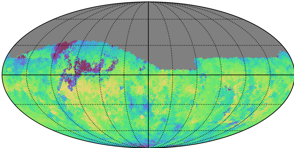
weather_cloudso4v3.4_10yrs Yr 1 z band: Median skyBrightness
