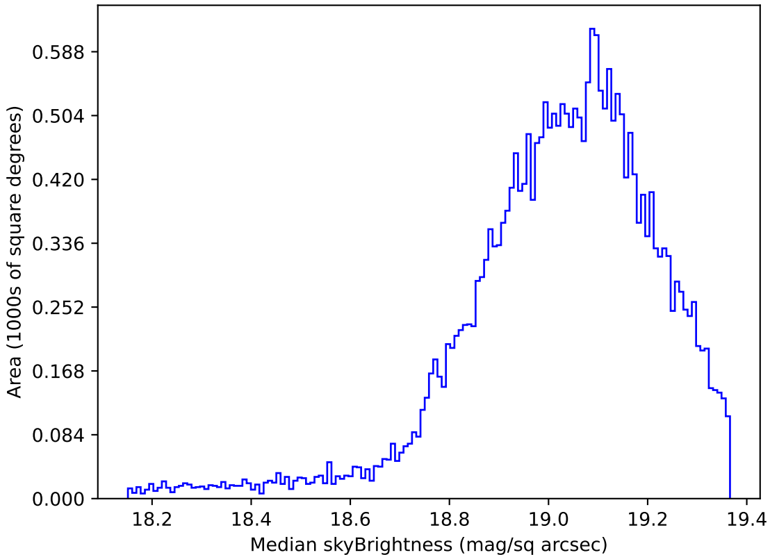
weather_cloudso4v3.4_10yrs Yr 1 z band: Median skyBrightness
